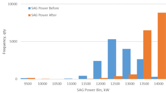
Figure 10 - SAG Power Bin
