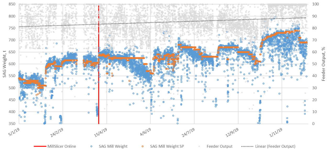
Figure 18 - SAG Weight Control and Feeder Output
