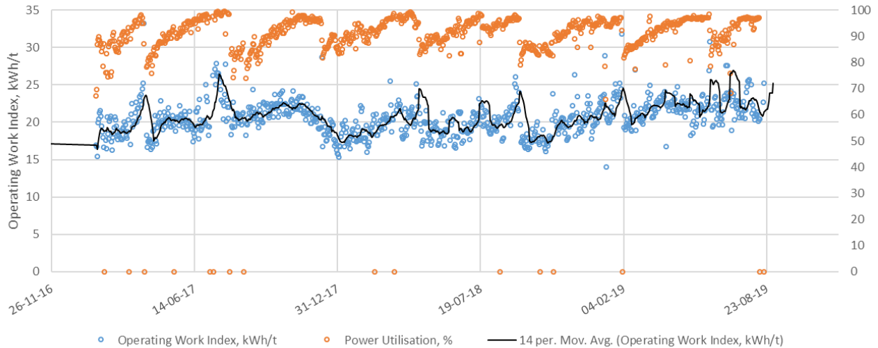
Figure 5 - Operating Work Index (Wio) vs. Time Relationship
