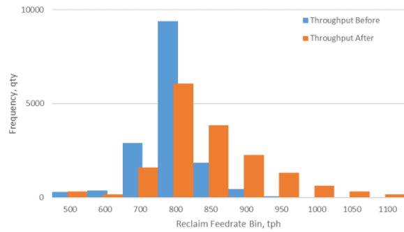
Figure 11 - Reclaim Feedrate Bin
