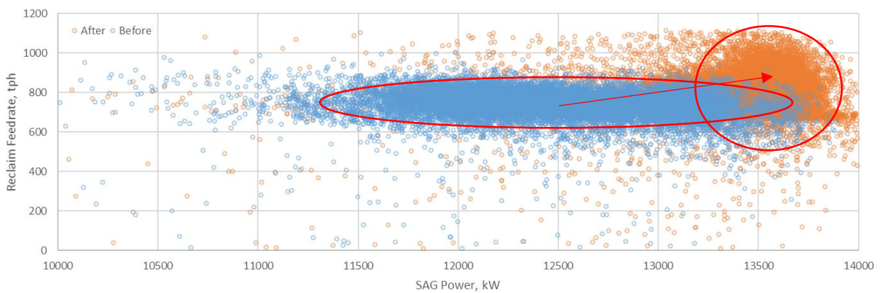
Figure 16 - Circuit Reclaim Throughput vs. SAG Power (5-minute instantaneous average)
