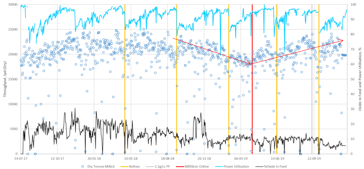
Figure 3 - Long Term Throughput Data
