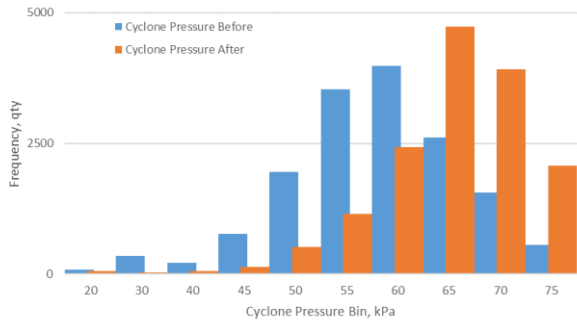
Figure 12 - Cyclone Pressure Bin
