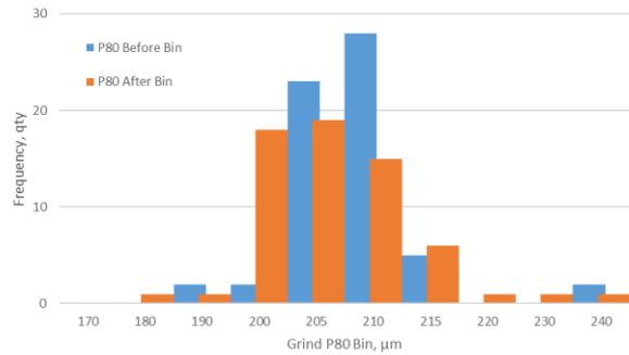
Figure 13 - Circuit Grind P 80
