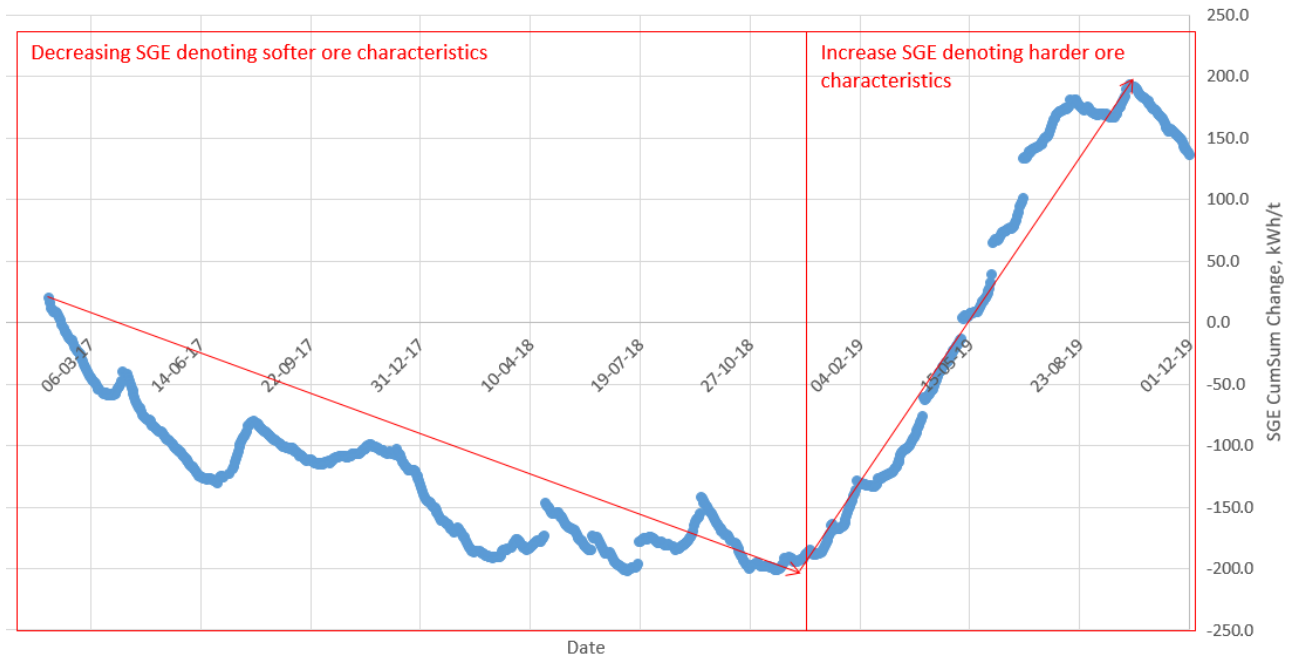
Figure 6 - SAG Mill Specific Grinding Energy Cumulative Sum
