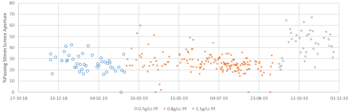
Figure 17 - Primary Crusher Product Fines Content
