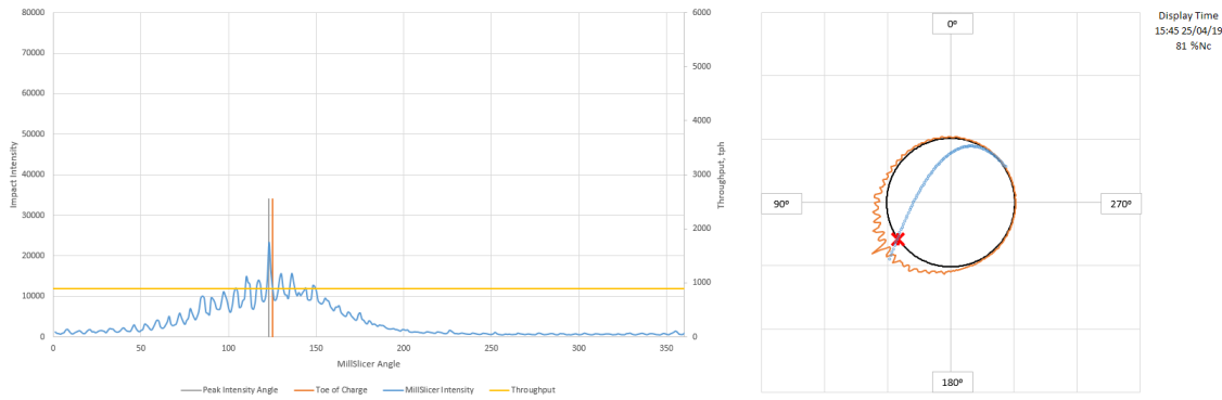
Figure 15 - MillSlicer Impact Intensity After (25 April 2019)
