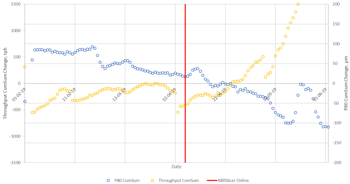
Figure 8 - Comparative Throughput Rate and Circuit Grind P_{80}
