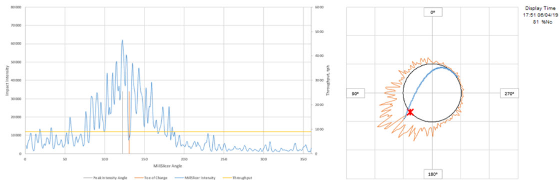
Figure 14 - MillSlicer Impact Intensity Before (06 April 2019)
